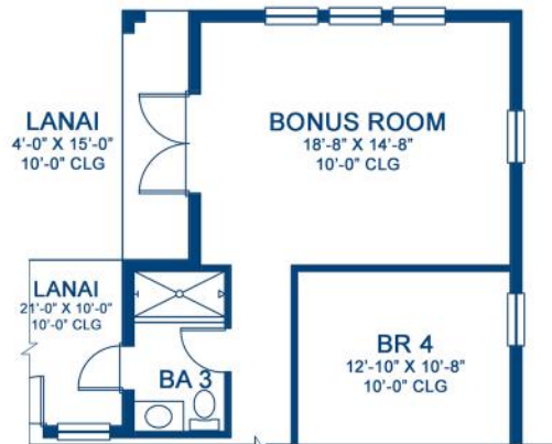
OPT. BONUS DOWNSTAIRS (+340 A/C S.F. +60 S.F. AT LANAI)
